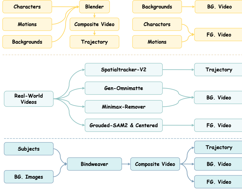
Fig. S2. Illustration of our data pipeline.
